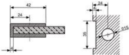
Glass cut - out top and bottom
