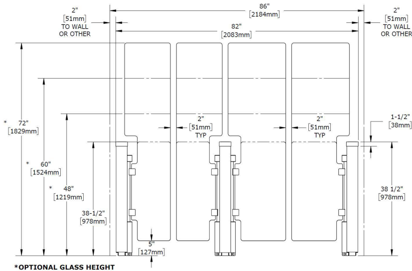
Typical SG200, SQ & RND Ends Standard / ADA 2 Lanes / 3 Ped
