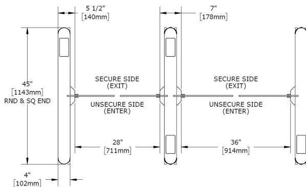
Typical SG200, SQ & RND Ends Standard / ADA 2 Lanes / 3 Ped
