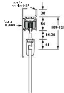
Pacer bracket
