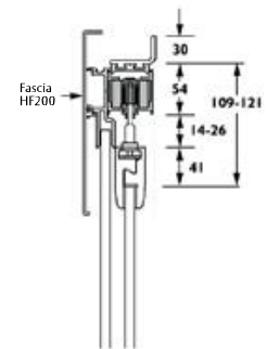
Pacer fixed panel fascia bracket
