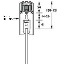
Pacer double fascia
