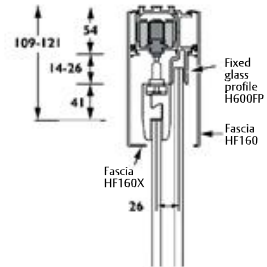
Pacer fixed panel
