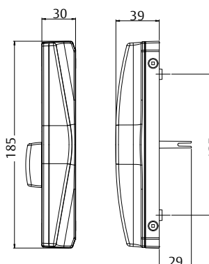
Snib & Cylinder
