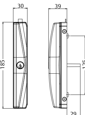
Double Cylinder
