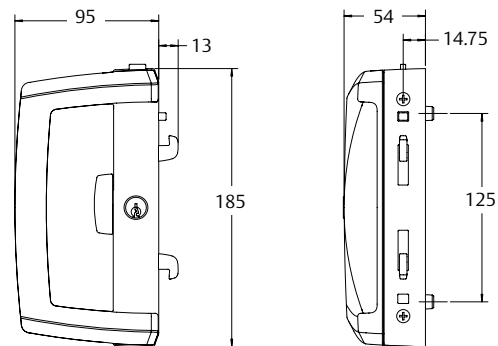
Interior D-Handle
