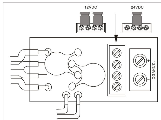
Wiring Diagram
