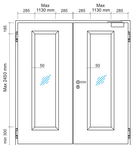
Maximum single pane – next to handle
