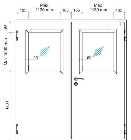
Maximum single pane - top
