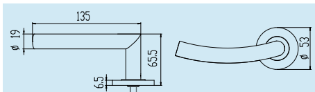
L90-shape curved lever AH123109
