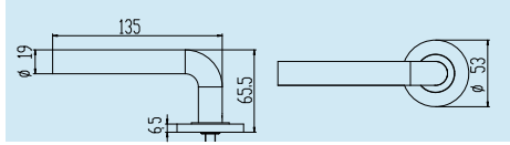
L-shape lever AH123102
