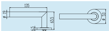
L90-shape lever AH123104
