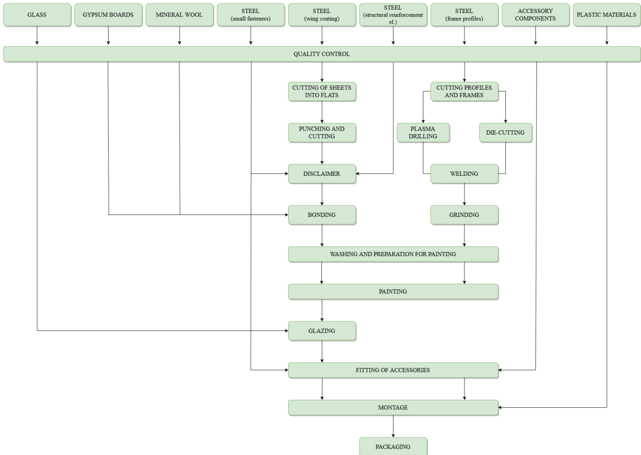
Fig. 1. A basic scheme of ALPE W manufacturing process
