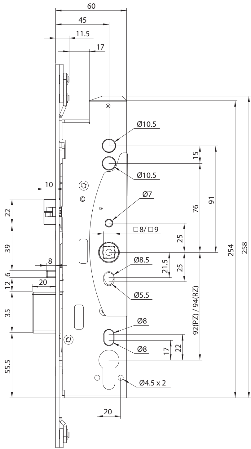
DETAIL A SCALE 1 : 2
