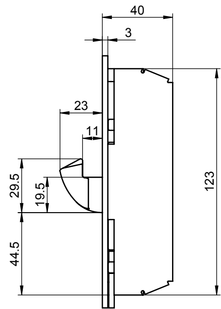
DETAIL B SCALE 1 : 2
