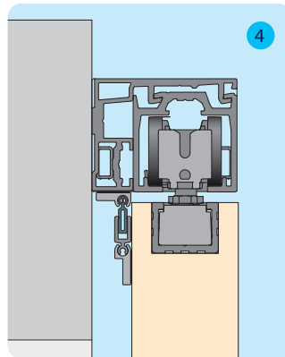
4. Wall mounting with variant A-B glued on the outside
