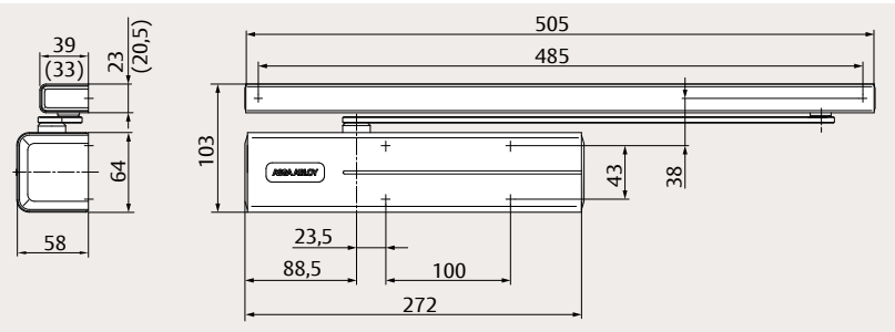
DC700, G195 (G193) dimensions in mm
