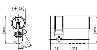
XCY2X20 Single Cylinder
