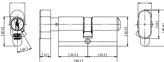
XCY2X19 Thumbturn Cylinder
