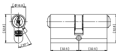
XCY2X18 Double Cylinder
