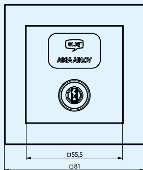
Frame mount
