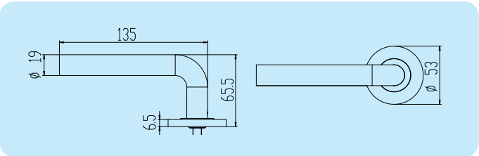
L-shape lever
