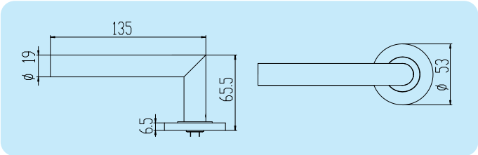
L90-shape lever
