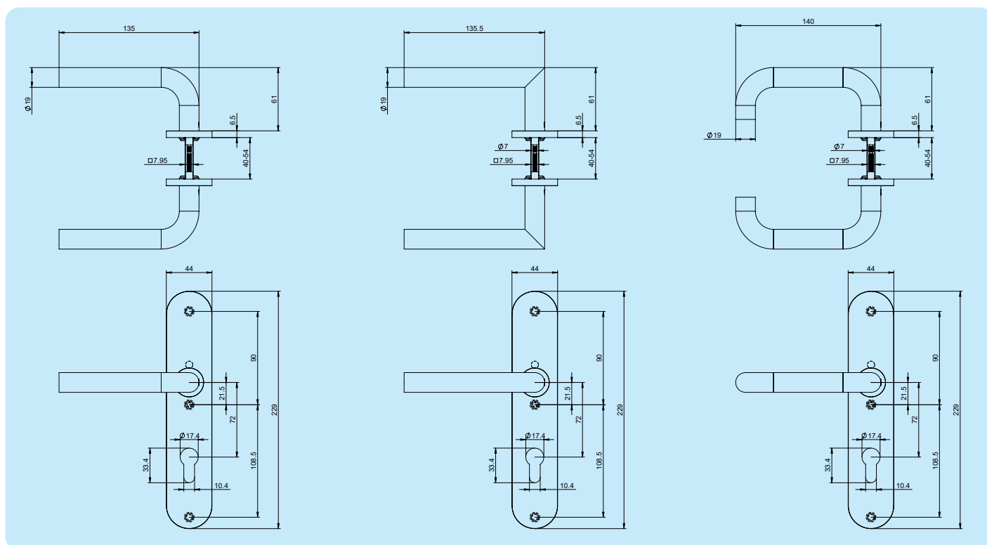
L-shape lever PC72* AH123402SSPC72
